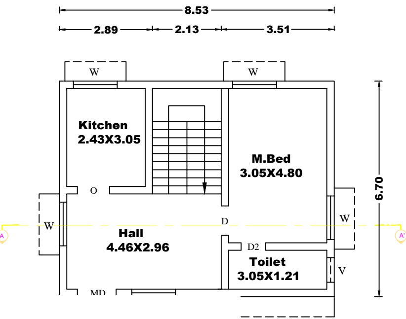
FLOOR PLAN
