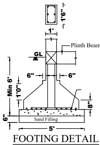
Column 0'9"x0'9" Not to Scale
