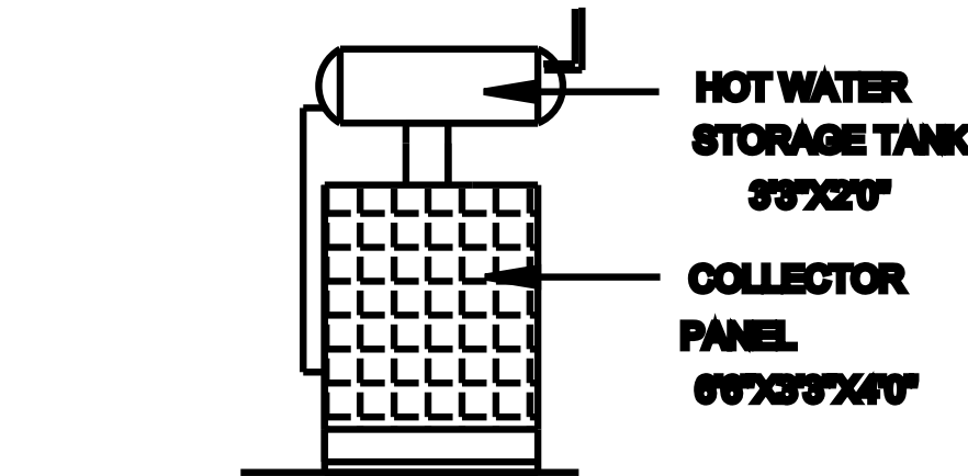
FRONT ELEVATION SOLAR WATER HEATER
