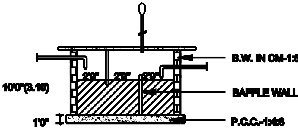
SEPTIC TANK SECTION-QC)
