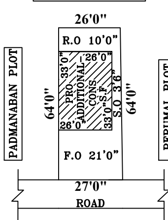
SITE PLAN
