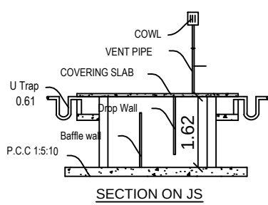
SECTION ON JJ'
