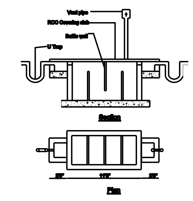
Rain Water Harvest Unit Not To Scale
