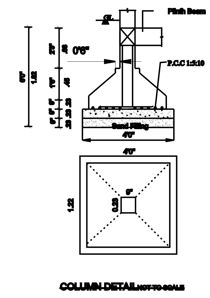
COLUMN DETAIL Not To Scale
