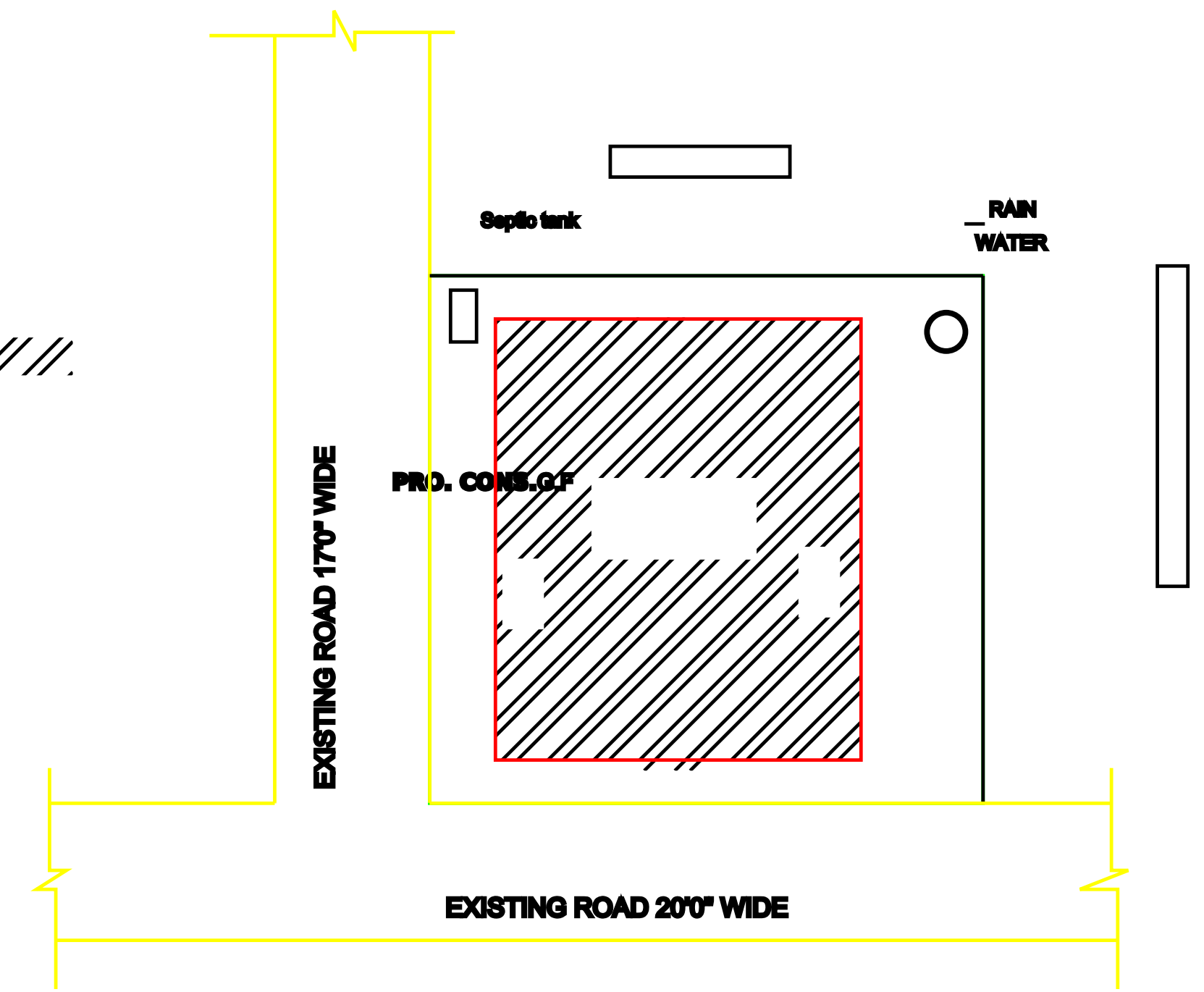
SITE PLAN SCALE - 1CM = 2M
