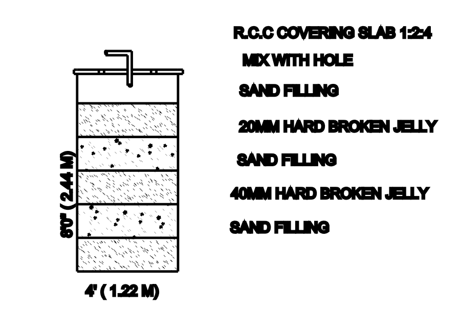
Rain Water Harvest Unit Not To Scale
