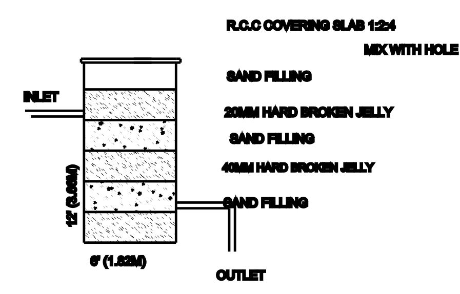
Rain Water Harvest Unit Not To Scale
