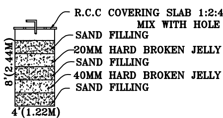
RAIN WATER HARVEST UNIT
