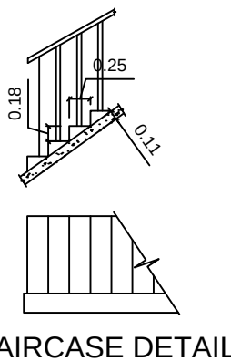
STAIRCASE DETAIL
