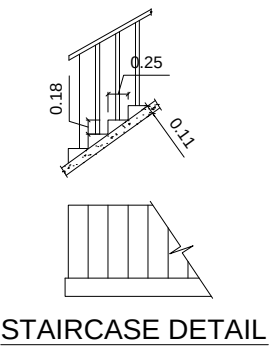
STAIRCASE DETAIL
