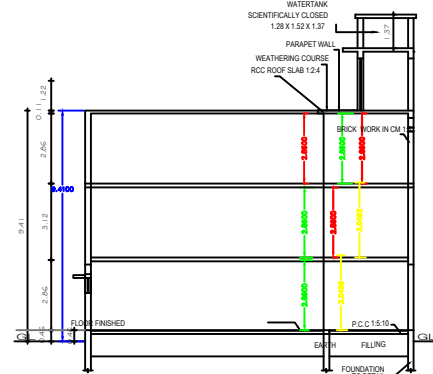
SECTION "A-B"
