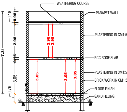
SECTION - AB'
