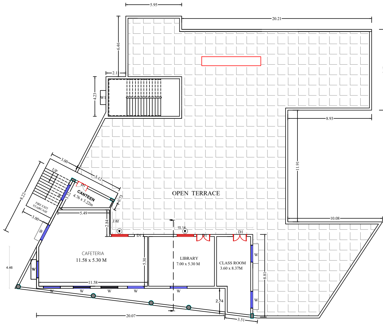
PRO.ADDI.CONST.FIRST FLOOR PLAN
