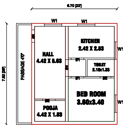
FIRST FLOOR PLAN RESIDENTIAL
