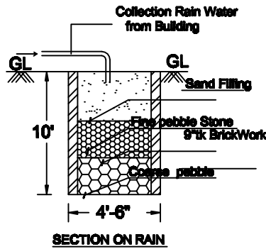
SECTION ON RAIN WATER COLLECTION TANK
