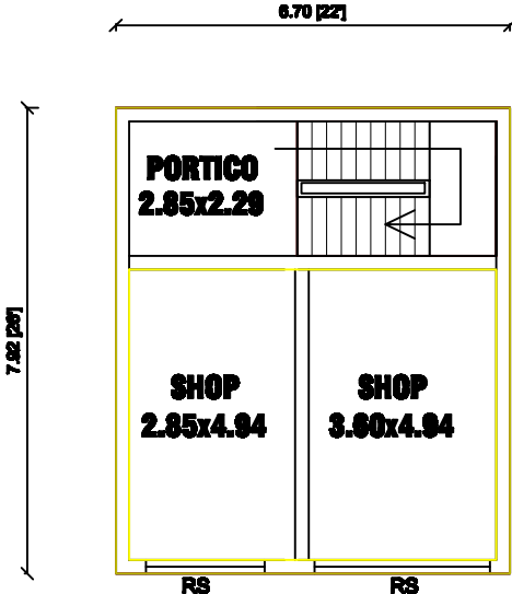
GROUND FLOOR PLAN COMMERCIAL
