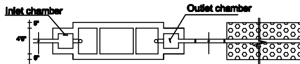
PLAN OF SEPTIC TANK AND DISPERSION TRENCH
