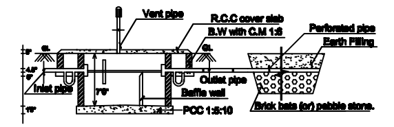
SECTION OF SEPTIC TANK AND DISPERSION TRENCH
