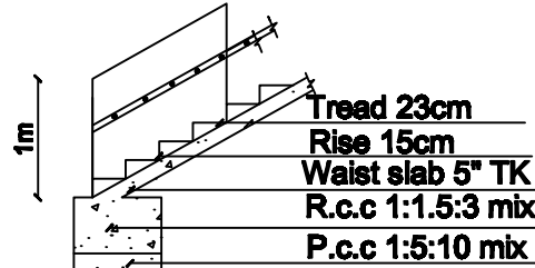
STAIRCASE DETAILS
