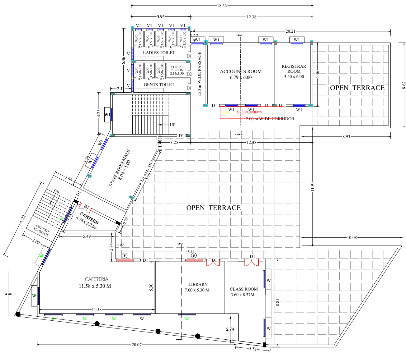
PRO.ADDI.CONST.FIRST FLOOR PLAN
