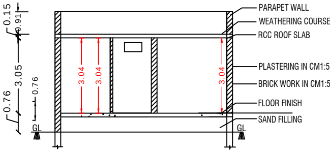
SECTION - AB'
