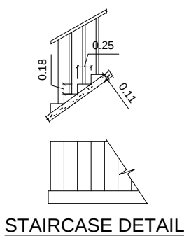
STAIRCASE DETAIL
