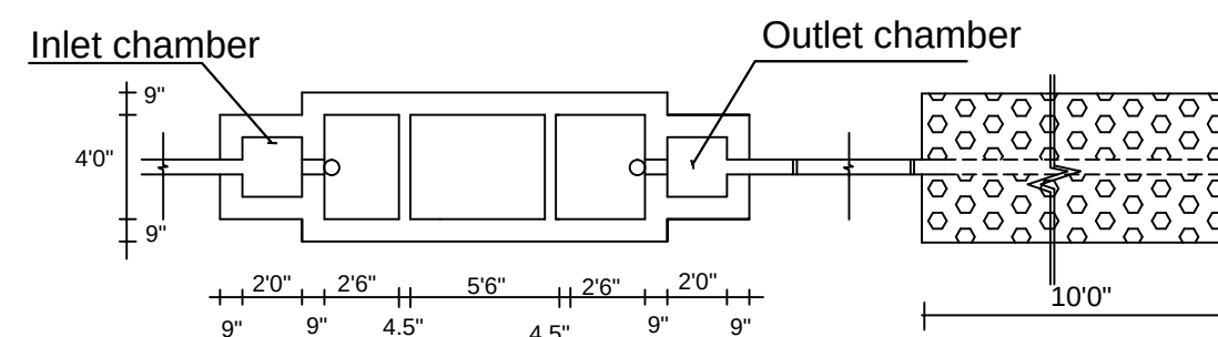
PLAN OF SEPTIC TANK AND DISPERSION TRENCH
