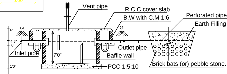
SECTION OF SEPTIC TANK AND DISPERSION TRENCH
