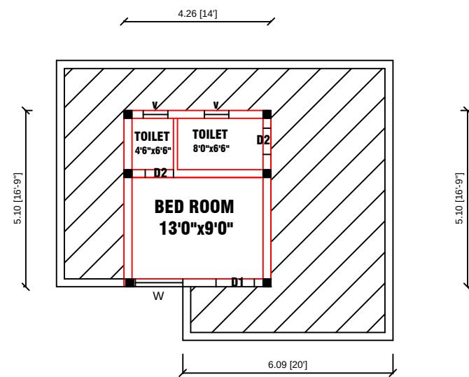
SECOND FLOOR PLAN RESIDENTIAL AC SHEET
