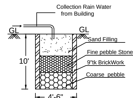
SECTION ON RAIN
