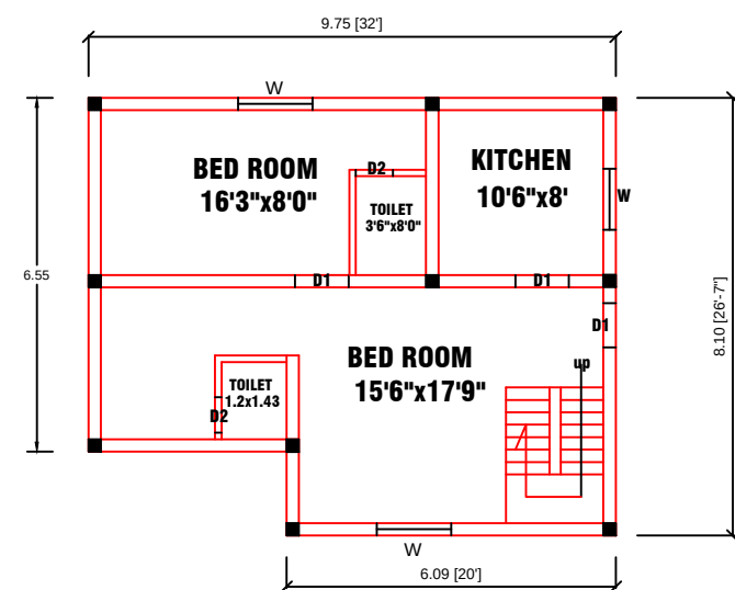
FIRST FLOOR PLAN RESIDENTIAL
