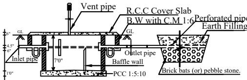
SECTION FOR SEPTIC TANK AND DISPERSION TRENCH
