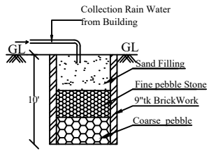
SECTION ON RAIN WATER COLLECTION TANK
