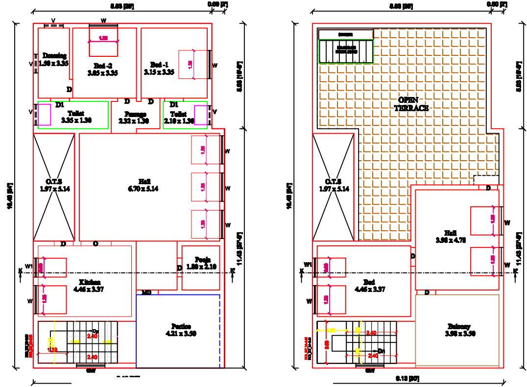
FIRST FLOOR & TERRACE PLAN
