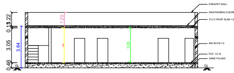
SECTION ON 'A-B'
