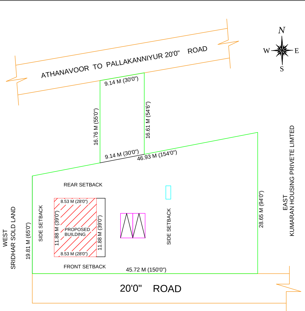
SITE PLAN
