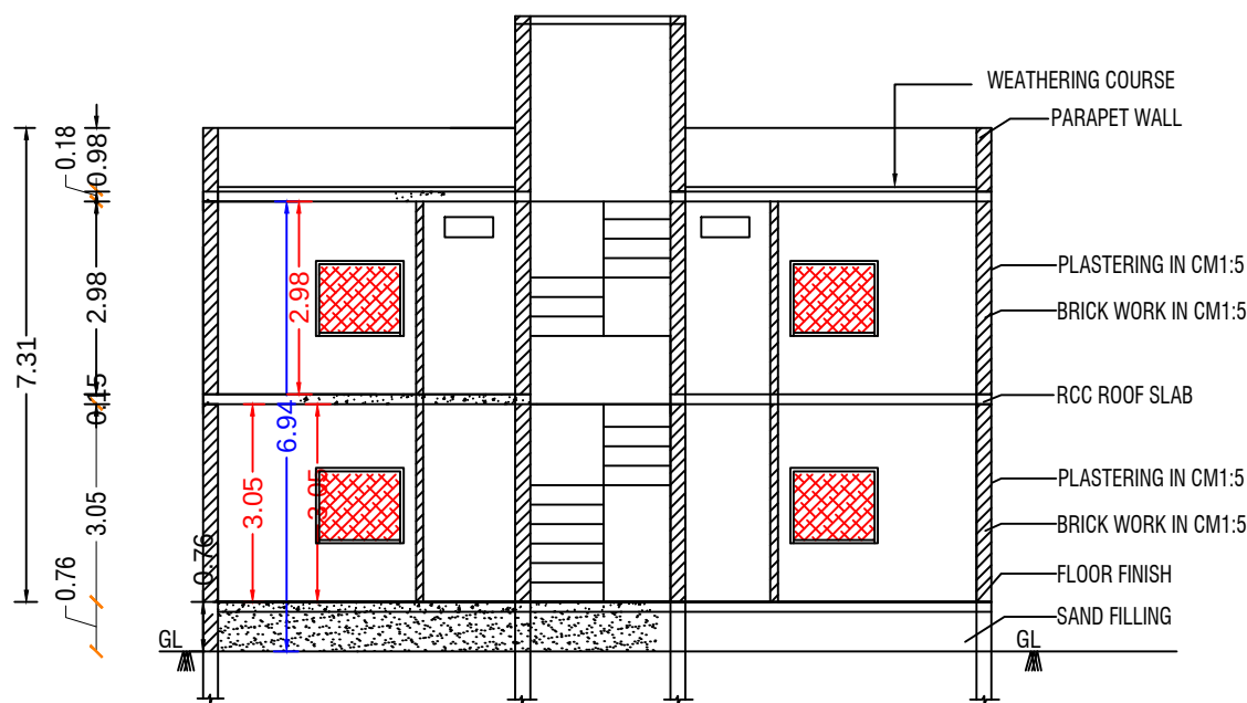
SECTION - AB'
