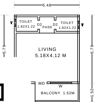
F FLOOR PLAN
