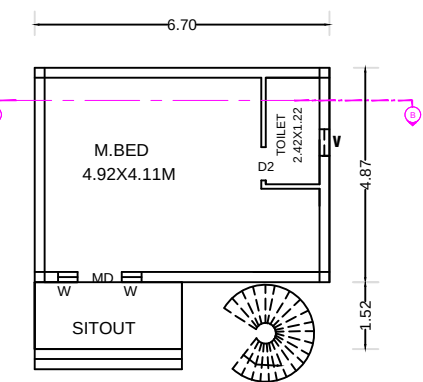
GROUND FLOOR PLAN BLOCK - 1
