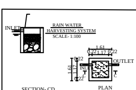
SECTION - CD
