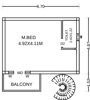
FIRST FLOOR PLAN BLOCK - 3
