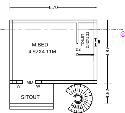
GROUND FLOOR PLAN BLOCK - 2
