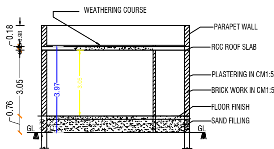
SECTION - CD'
