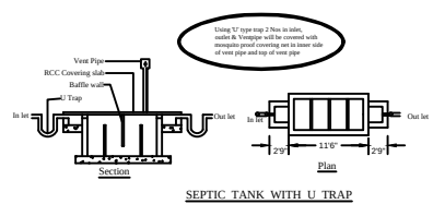
SEPTIC TANK WITH U TRAP
