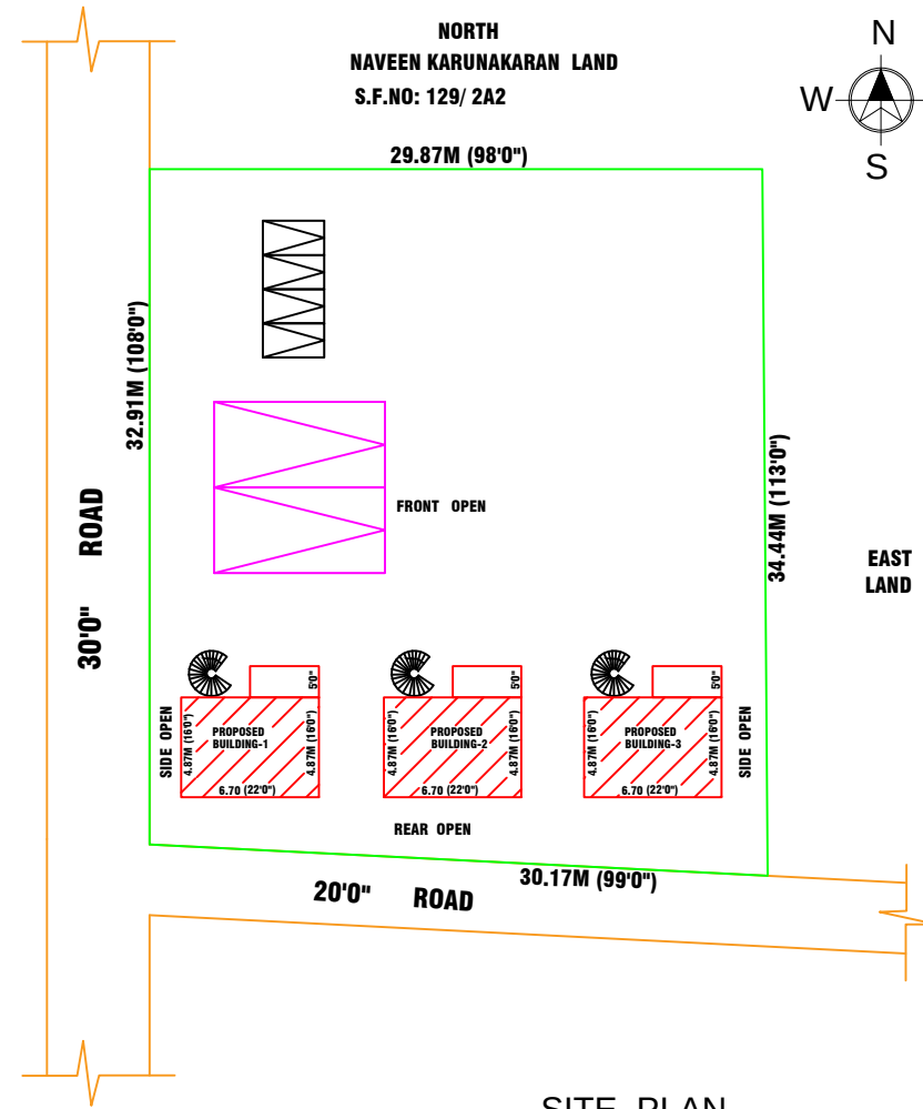
SITE PLAN
