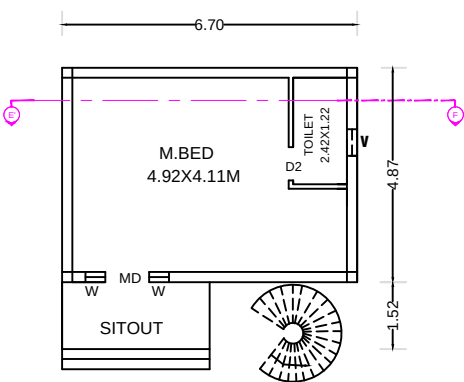
GROUND FLOOR PLAN BLOCK - 3
