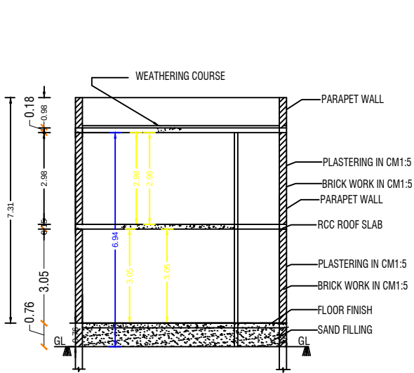
SECTION - AB'
