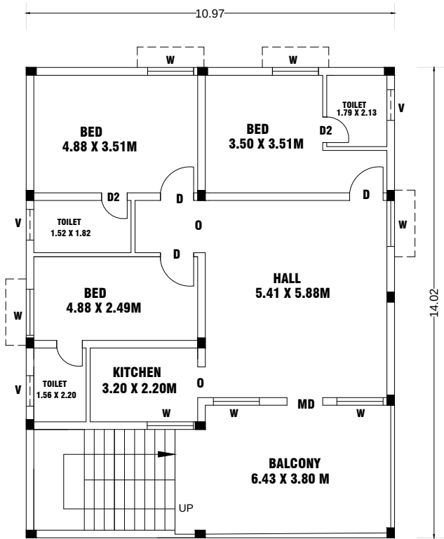
PROPOSED ADDI.CONT. FIRST FLOOR PLAN
