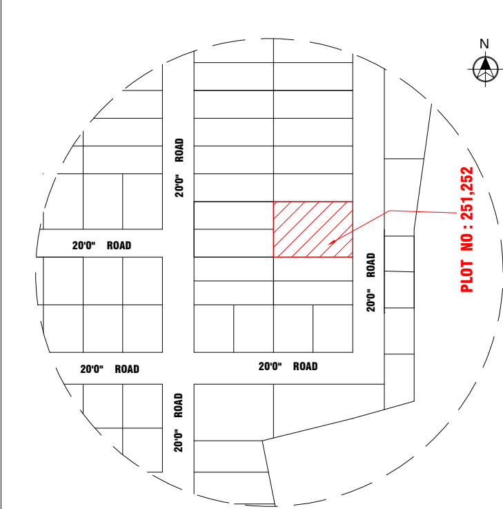
TOPO PLAN
