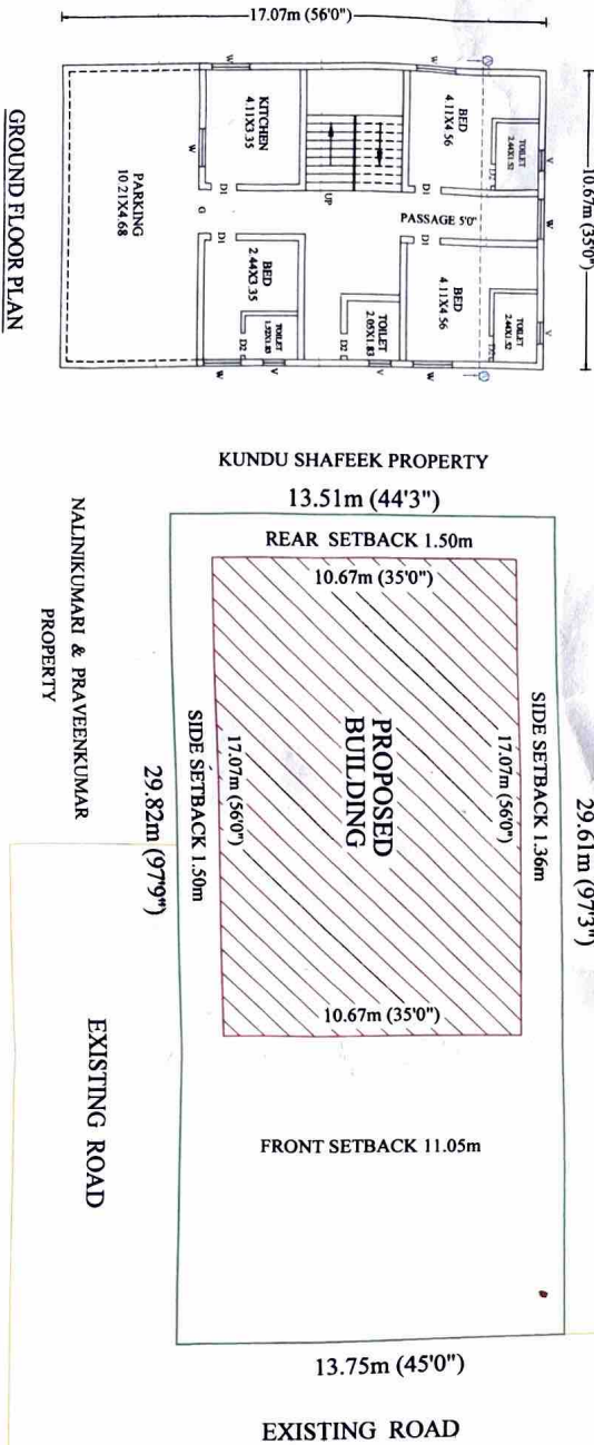
SITE PLAN
