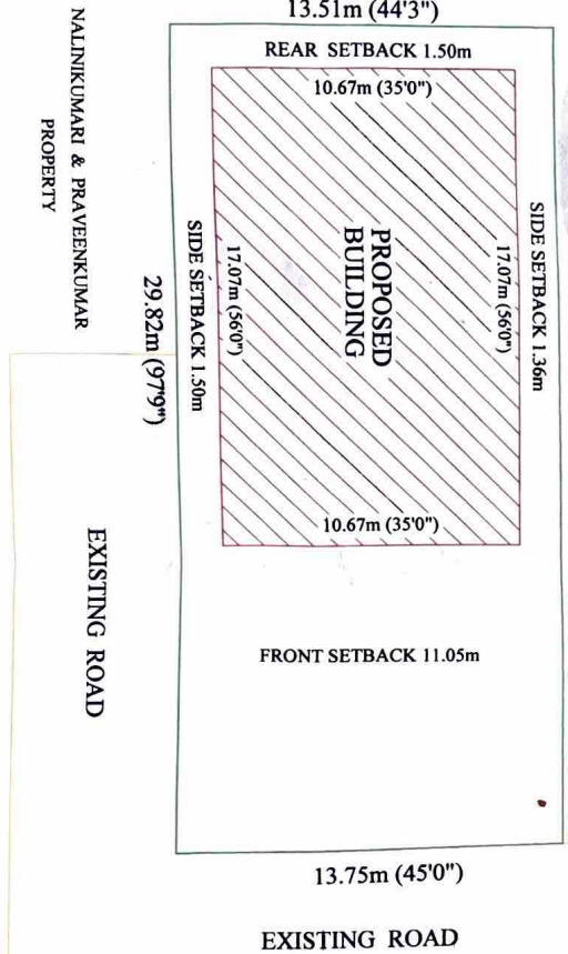
SITE PLAN
