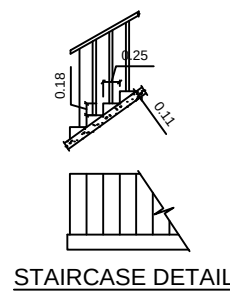
STAIRCASE DETAIL
