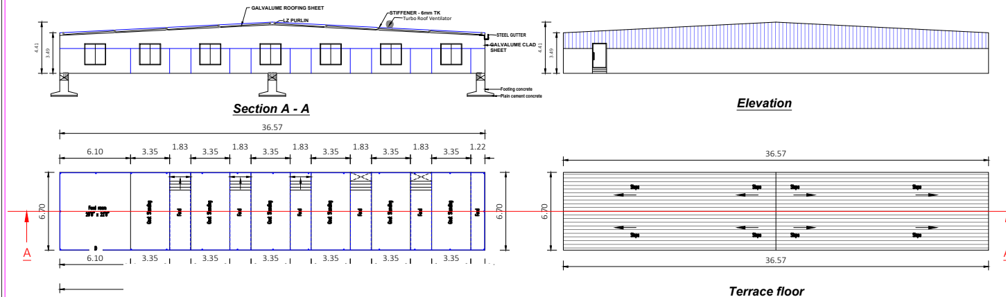
Terrace floor
