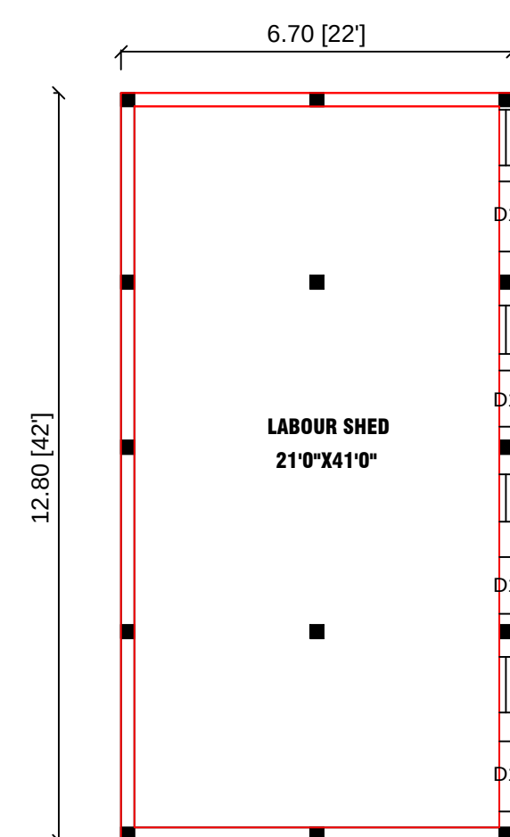
GROUND FLOOR PLAN LABOUR SHED
