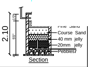
RAINWATER HARVESTING TANK SCALE 1:50
