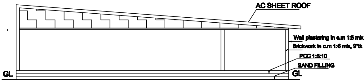
SECTION ON -AA
