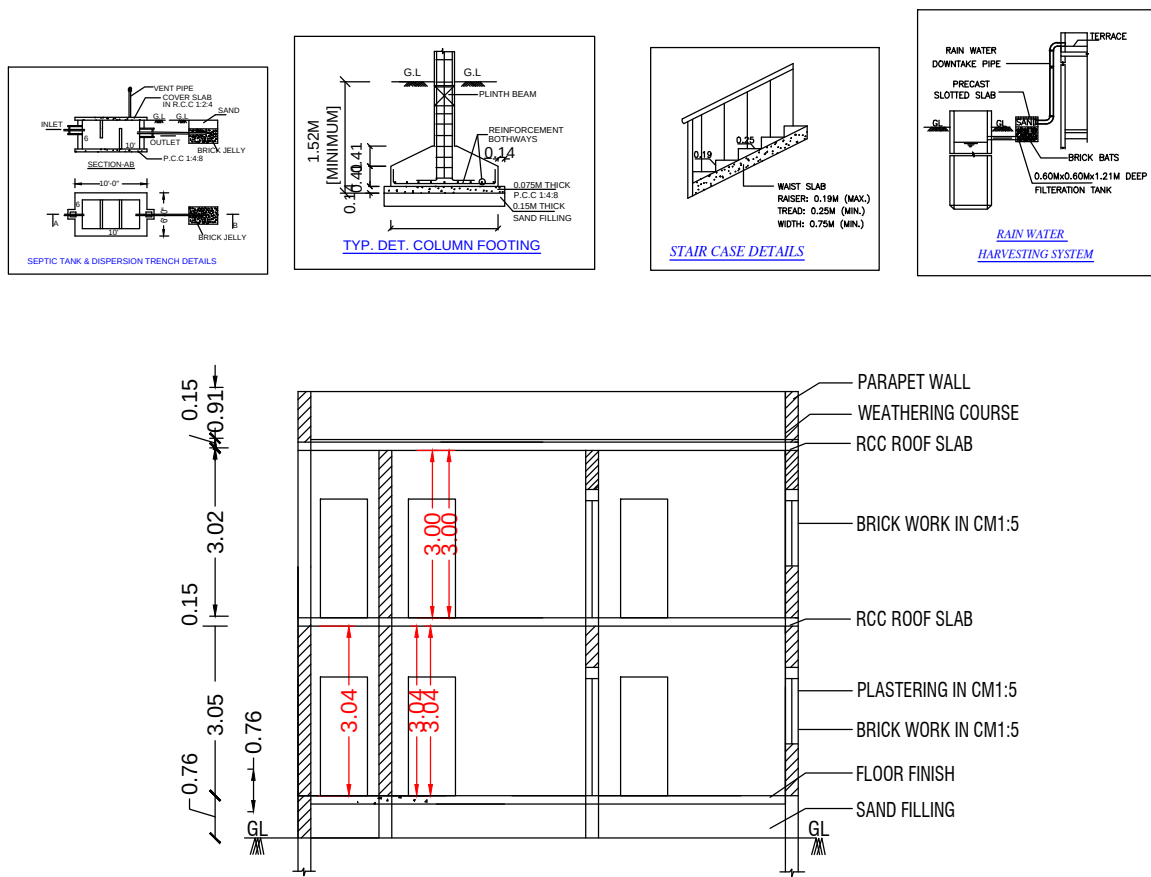
SECTION - AB'
