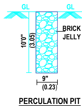
PERCOLATION PIT
