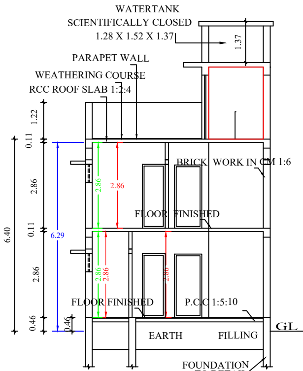
SECTION "A-B"
