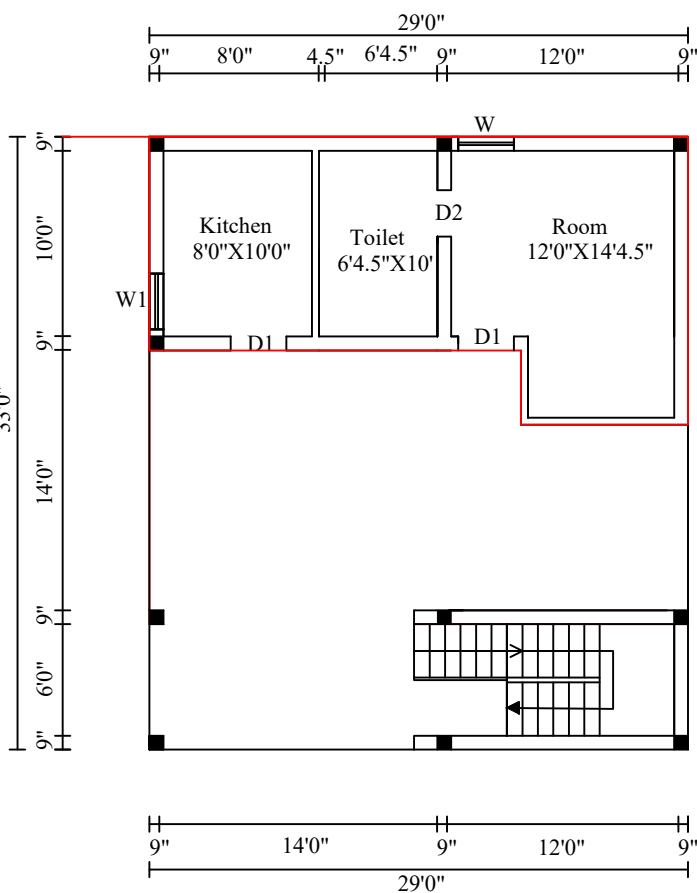
PROPOSED ADDITIONAL FIRST FLOOR PLAN
