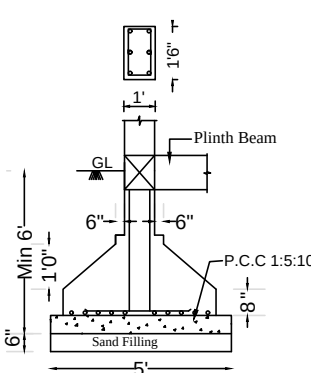
FOOTING DETAIL Column 0'9"x0'9" Not to Scale
