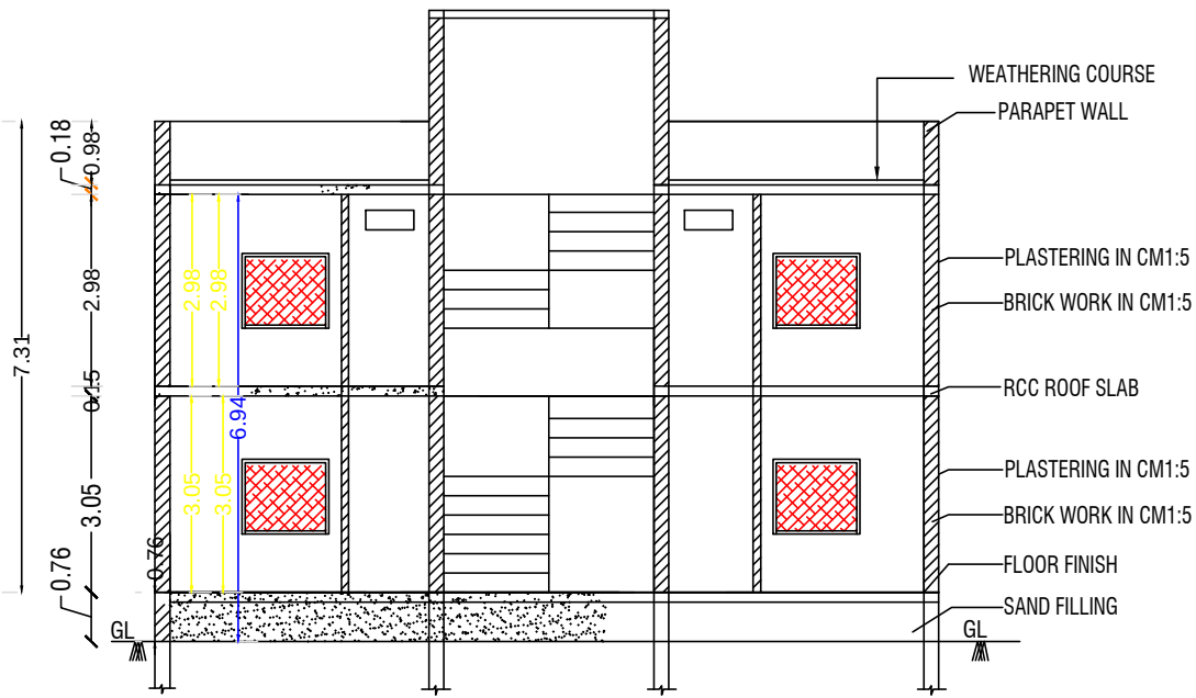
SECTION - AB'
