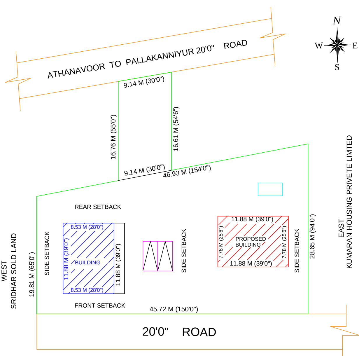
SITE PLAN
