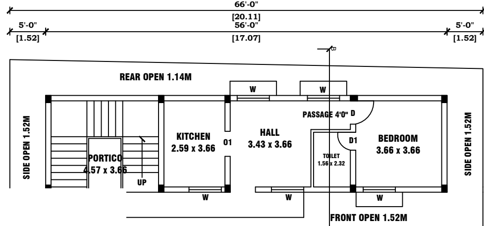
PROPOSED CONSTRUCTION FIRST FLOOR PLAN.
