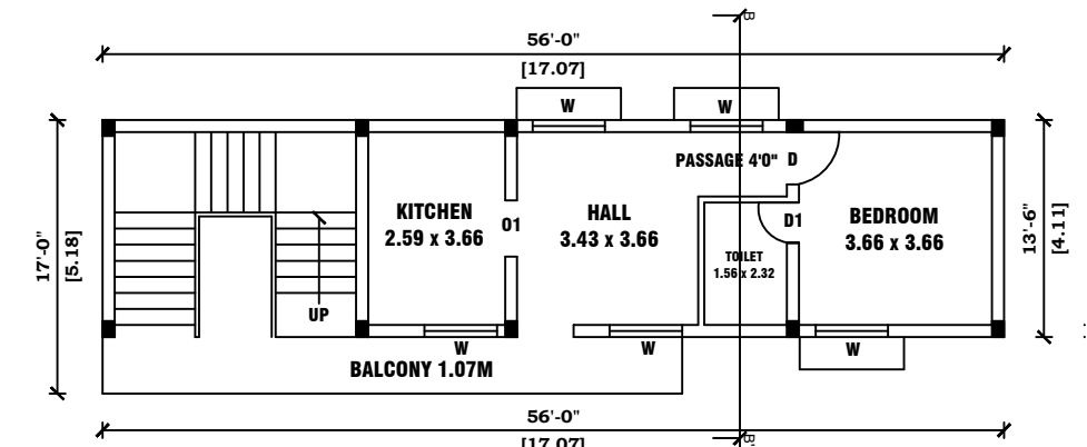
PROPOSED CONSTRUCTION FIRST FLOOR PLAN.
