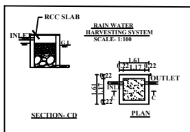
SECTION AND PLAN
