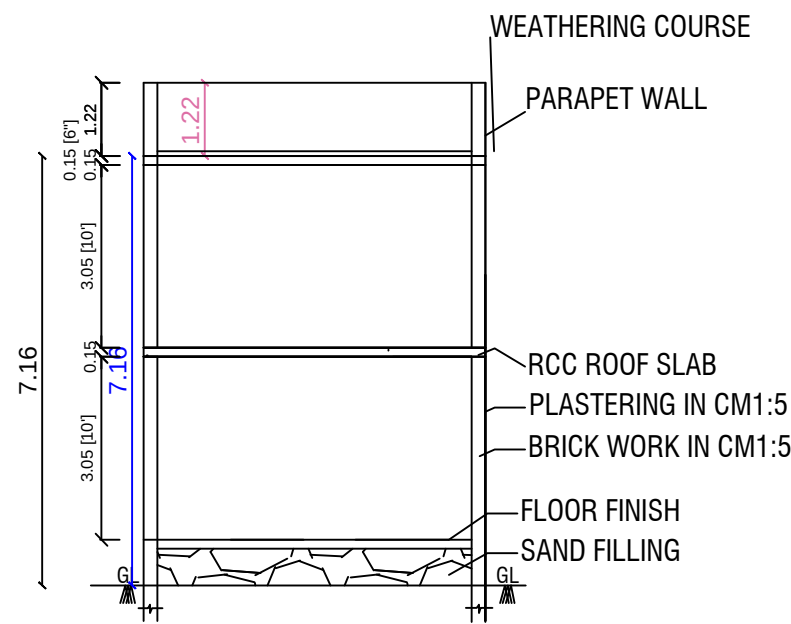
SECTION - AB'
