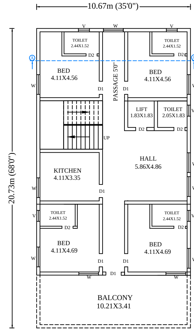
FIRST FLOOR PLAN (PROPOSED RESIDENTIAL BUILDING)
