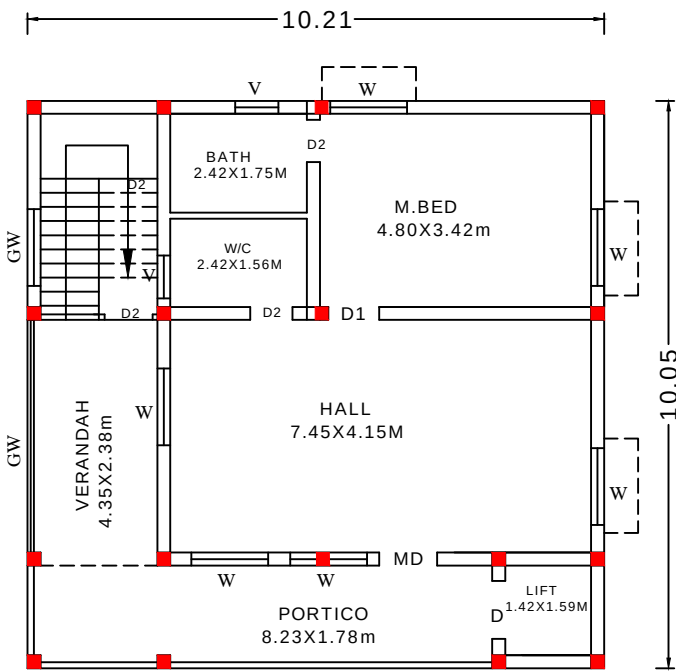
PRO.SECOND FLOOR PLAN
