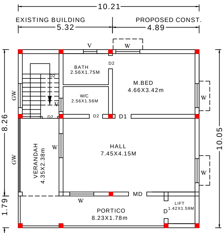
PROPOSED ADDIT.CONST. FIRST FLOOR PLAN
