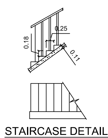
STAIRCASE DETAIL
