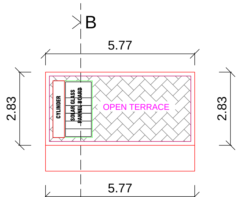
OPEN TERRACE PLAN
