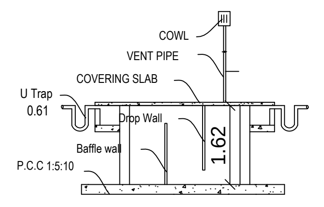
SECTION ON JS
