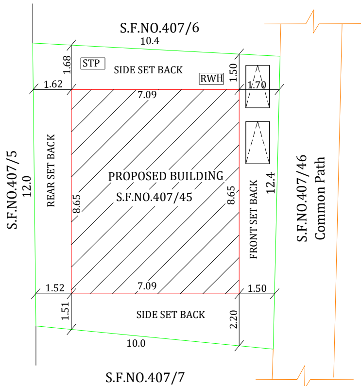
SITE PLAN
