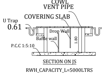
RWH_CAPACITY_L=5000LTRS
