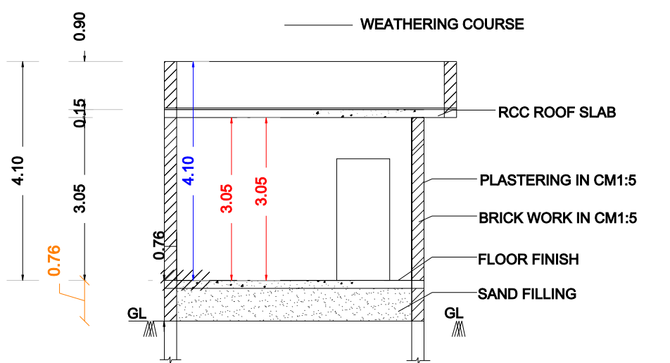
SECTION - AB'
