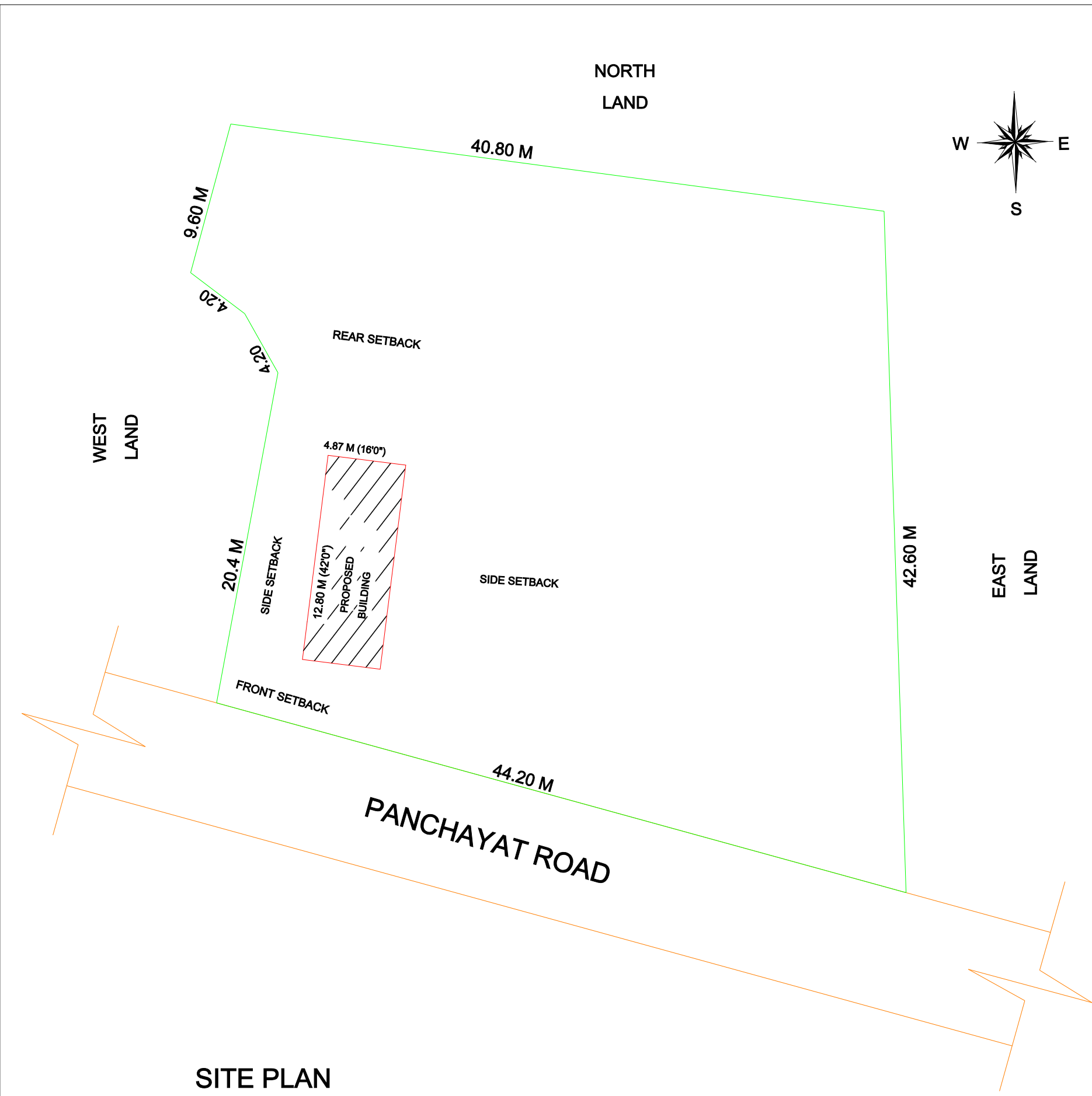
SITE PLAN
