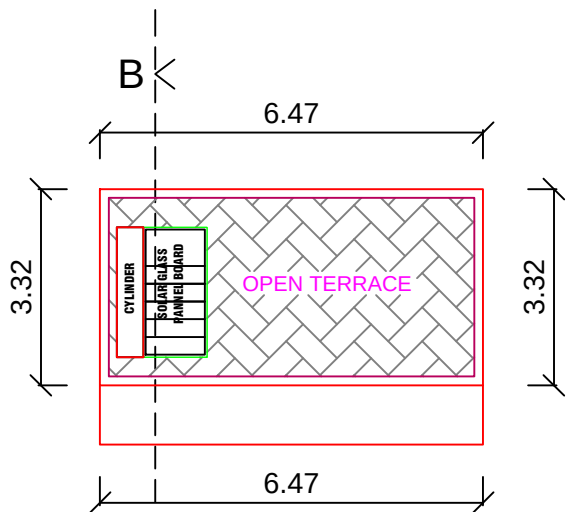
OPEN TERRACE PLAN
