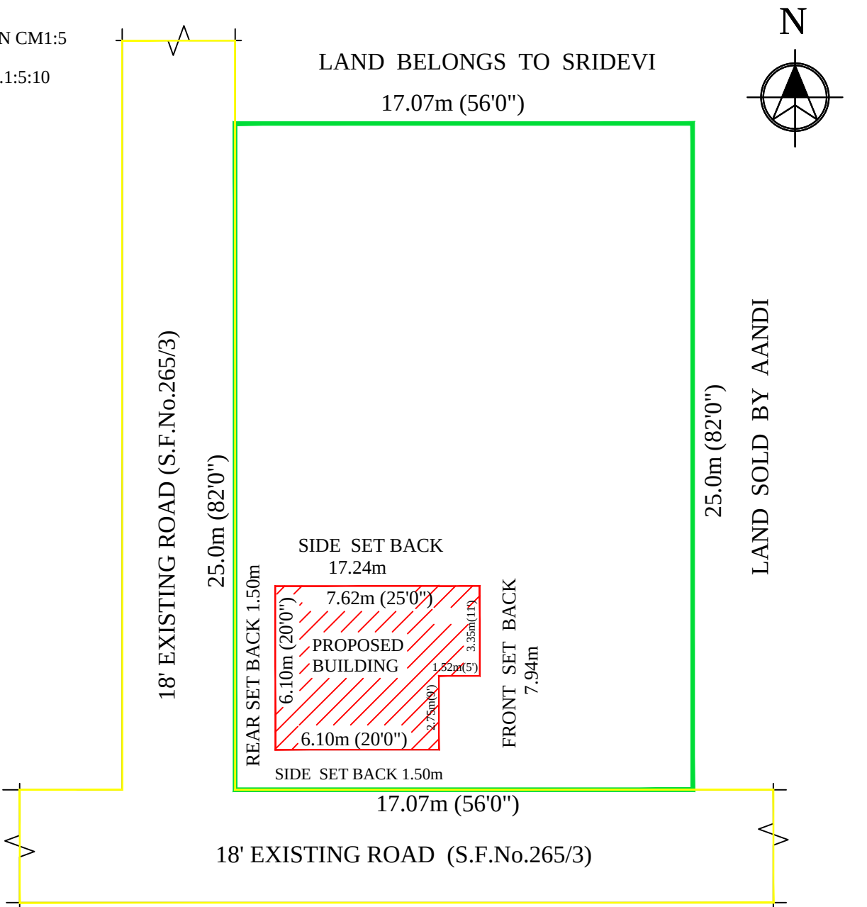
SITE PLAN
