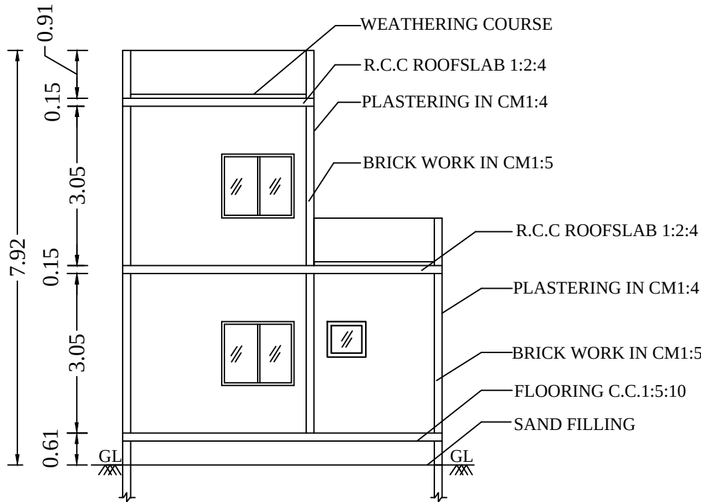
SECTION
