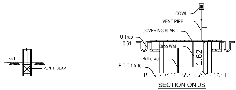
SEPTIC TANK DETAILS 'U' type trap 2 Nos in inlet, outlet pipe will be covered with Mosquito net in inner side and top of vent.
