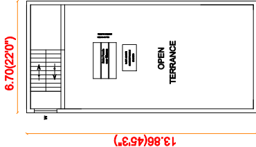
TERRACE FLOOR PLAN
