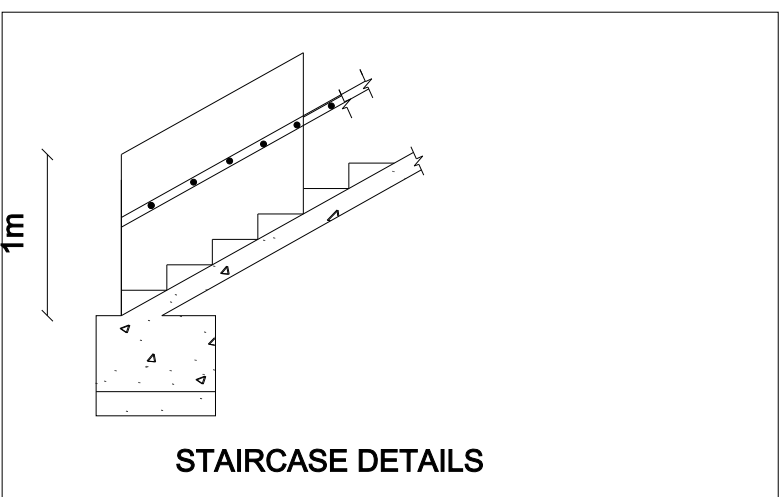
STAIRCASE DETAILS
