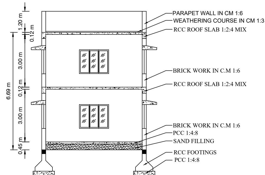
SECTION-AB
