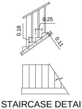
STAIRCASE DETAIL
