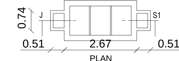
SEPTIC TANK DETAILS
