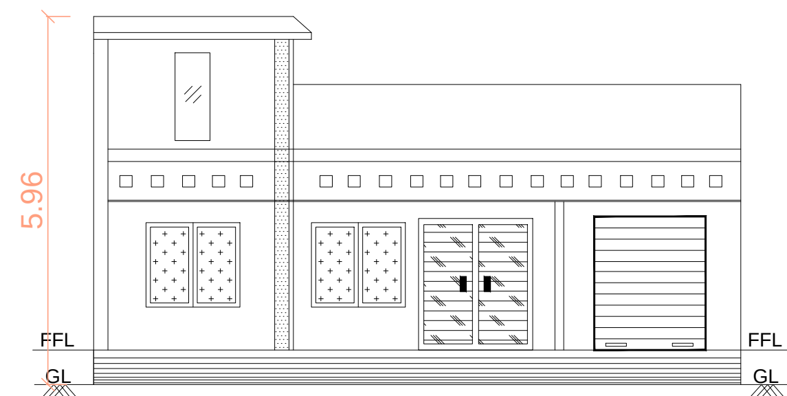
FRONT ELEVATION
