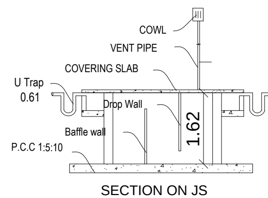
SECTION ON 'J-S'
