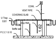
SECTION ON 'AB'
