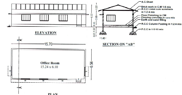
PLAN BLOCK - 2
