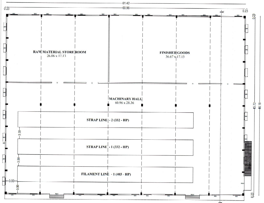
PLAN BLOCK - 1
