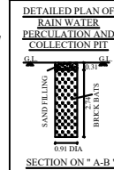
SECTION ON "A-B"
