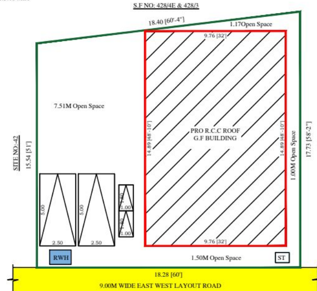
SITE PLAN (1:100)
